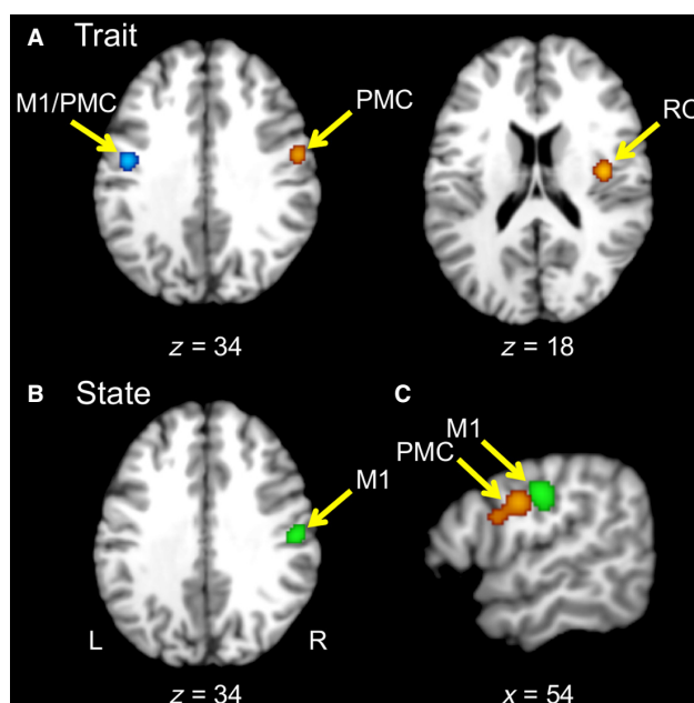
FIG. 1. Results of the ALE re-analysis. Axial slices in neurological convention showing regions consistently reported for (A) trait over-activations (red) and trait under-activations (blue), and (B) state over-activations (green). (C) Sagittal view highlighting trait over-activations in orofacial premotor cortex, and state over-activation in orofacial primary motor cortex. Peak coordinates and extent of activation cover the approximate somatotopic representations of the laryngeal and lip muscles. M1, primary motor cortex; PMC, premotor cortex; RO, Rolandic operculum. [Colour figure can be viewed at wileyonlinelibrary.com ].
